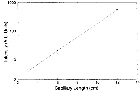
FIG. 3. Integrated line intensity of the J = 0-1 line of Ar IX as a function of the plasma column length. A fit to the Linford formula [26] yields a gain coefficient of 0.6 \pm 0.04 \text{cm}^{-1} , corresponding to gl = 7.2 .
